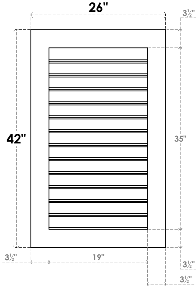
FRONT
